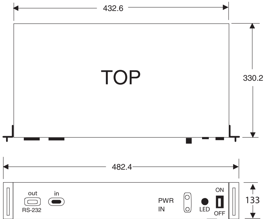
FRONT PANEL
